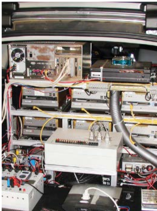
LOW BUDGET: Maahesh Chengalva wrote all the code for the low-budget, high-ambition Ody-Era (#55). Other robot cars had so much computer power that they required onboard gen-sets for power and air conditioning.
