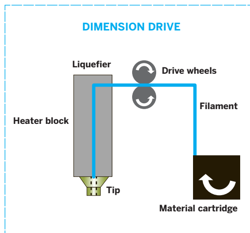
CLOCKWISE FROM LEFT: The Fab@Home extruder is a syringe driven by a linear actuator; the Stratasys Dimension 3D printer extrudes a filament of heated plastic; the author's DIY cookie press, retrofitted for computer control with a $6 motor.
