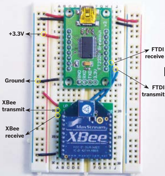
Fig. F: XBee module on the breakout board, wired to a general-purpose USB-to-TTL serial adapter. Fig. G: The Simple Processing application graphs accelerometer readings and counts a collision when
