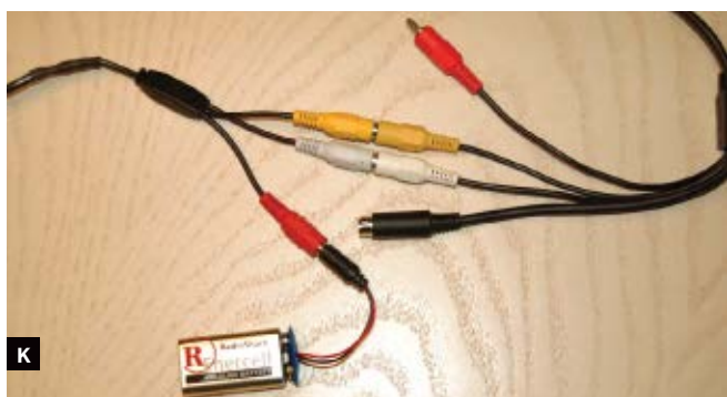
Fig. J: Use hot glue to secure the webcam to the sunglasses. Hold the camera in place until the glue solidifies completely. Fig. K: Plug the cable into the camcorder and attach the 9V battery.
