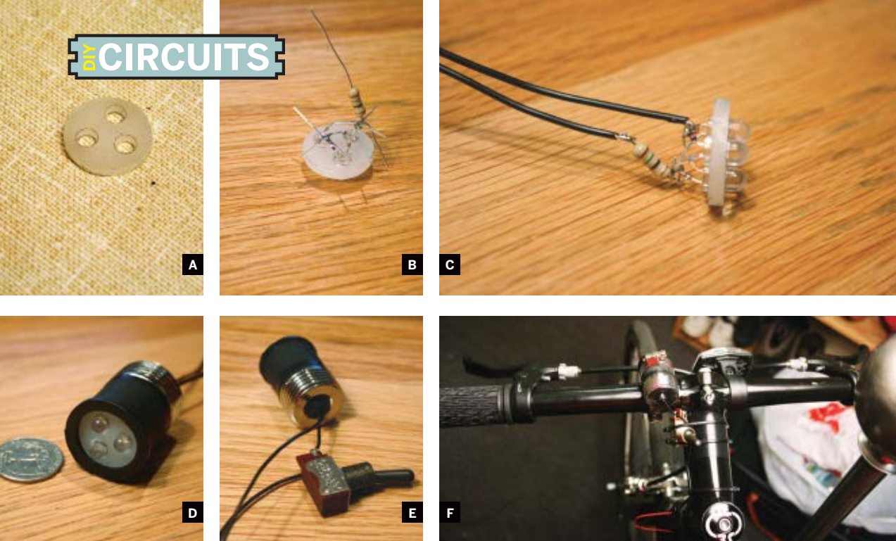
Fig. A: Drilled plastic disk for holding LEDs. Fig. B: LEDs glued into the disk and wired together with the resistor. Fig. C: Leads connected for power and switch. Fig. D: LED disk fit into the rubber end of the faucet hose adapter.
