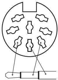
Mobile as modem: phone port to sub-mini jack.
