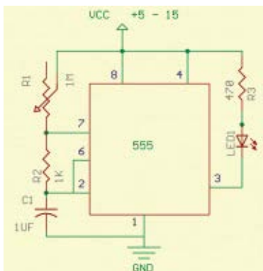
Schematic.
