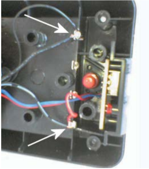
On the underside of the DTV's top half, we'll connect our power supply and the main board's keyboard power terminals to the battery contact terminals shown above.
