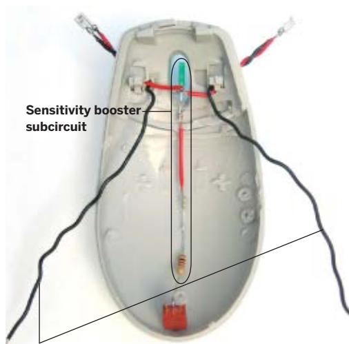
To Pins 2 and 3 of IC
