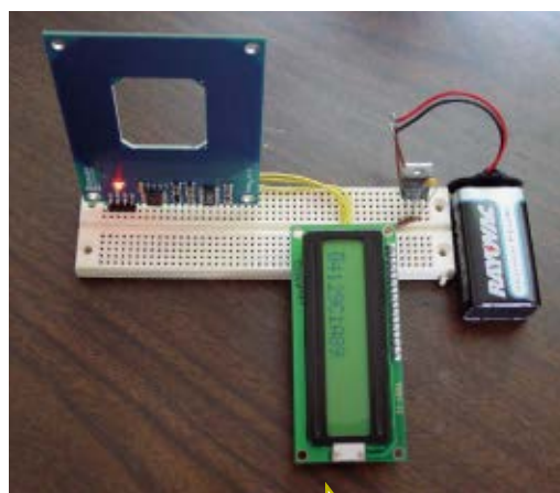
Figure 4. RFID reader module in action.
