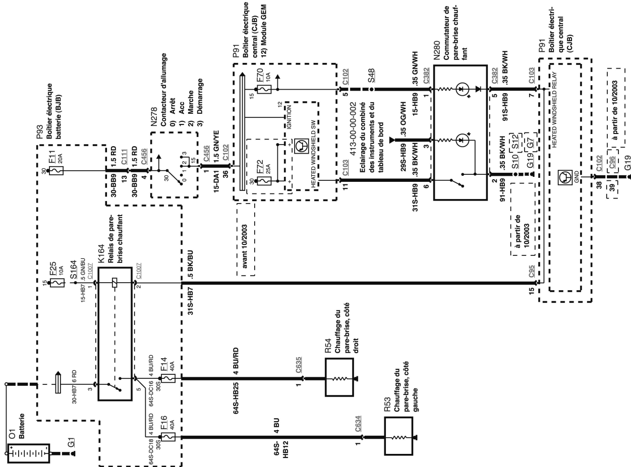
Pare-brise chauffant
