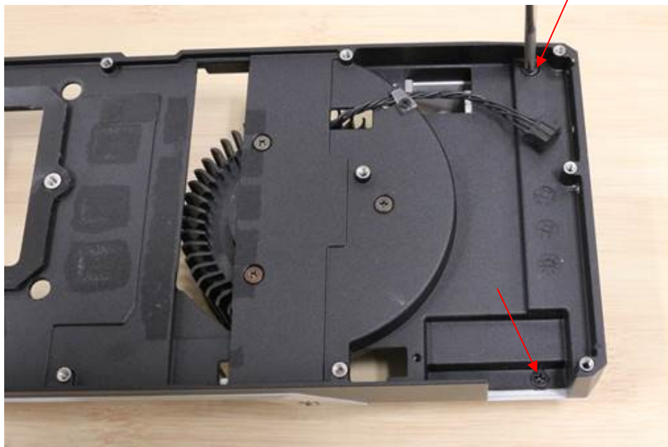
Figure 2f: At the bottom of the fansink base, secure the cover-right to baseplate with M2.5x5.0mm Philips wafer head screws (2X, black nickel). Torque screws to 3.0~3.5 in-lbf in sequence as indicated. Note: add Loctite 242 Threadlocker (3~5 threads from tip) if screw doesn't come with Nylok coating.
