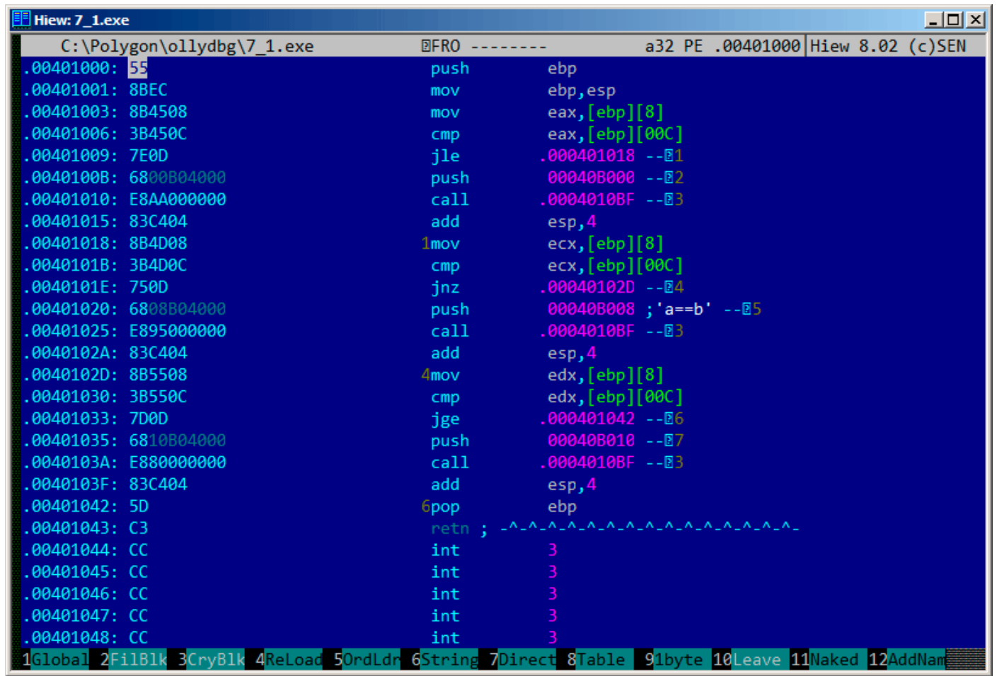
Figure 1.41: Hiew: f_unsigned() function
