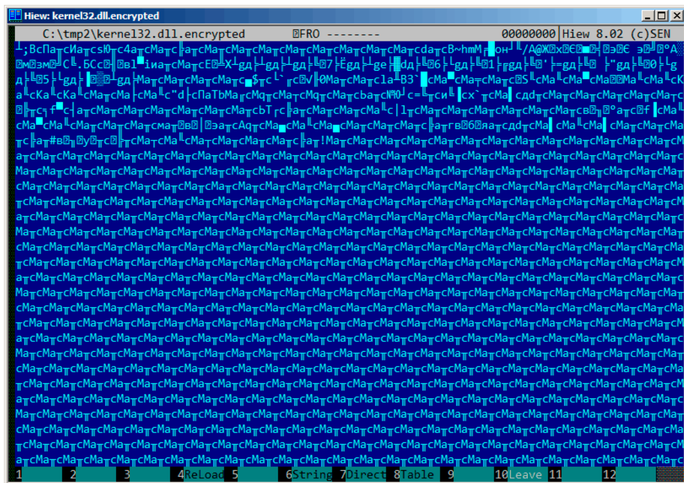
Figure 9.5: “Encrypted” file
