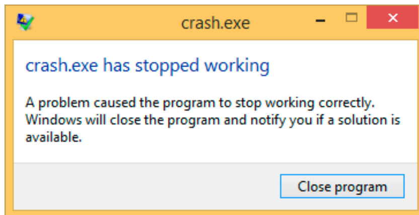
Figure 6.5: Windows 8.1
