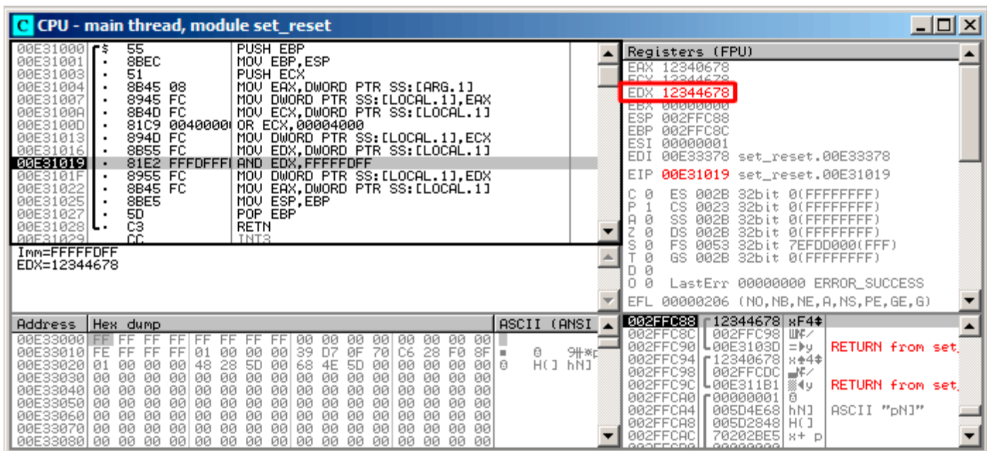
Figure 1.97: OllyDbg: value has been reloaded into EDX
