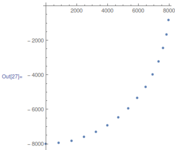
Figure 8.12: Mathematica
