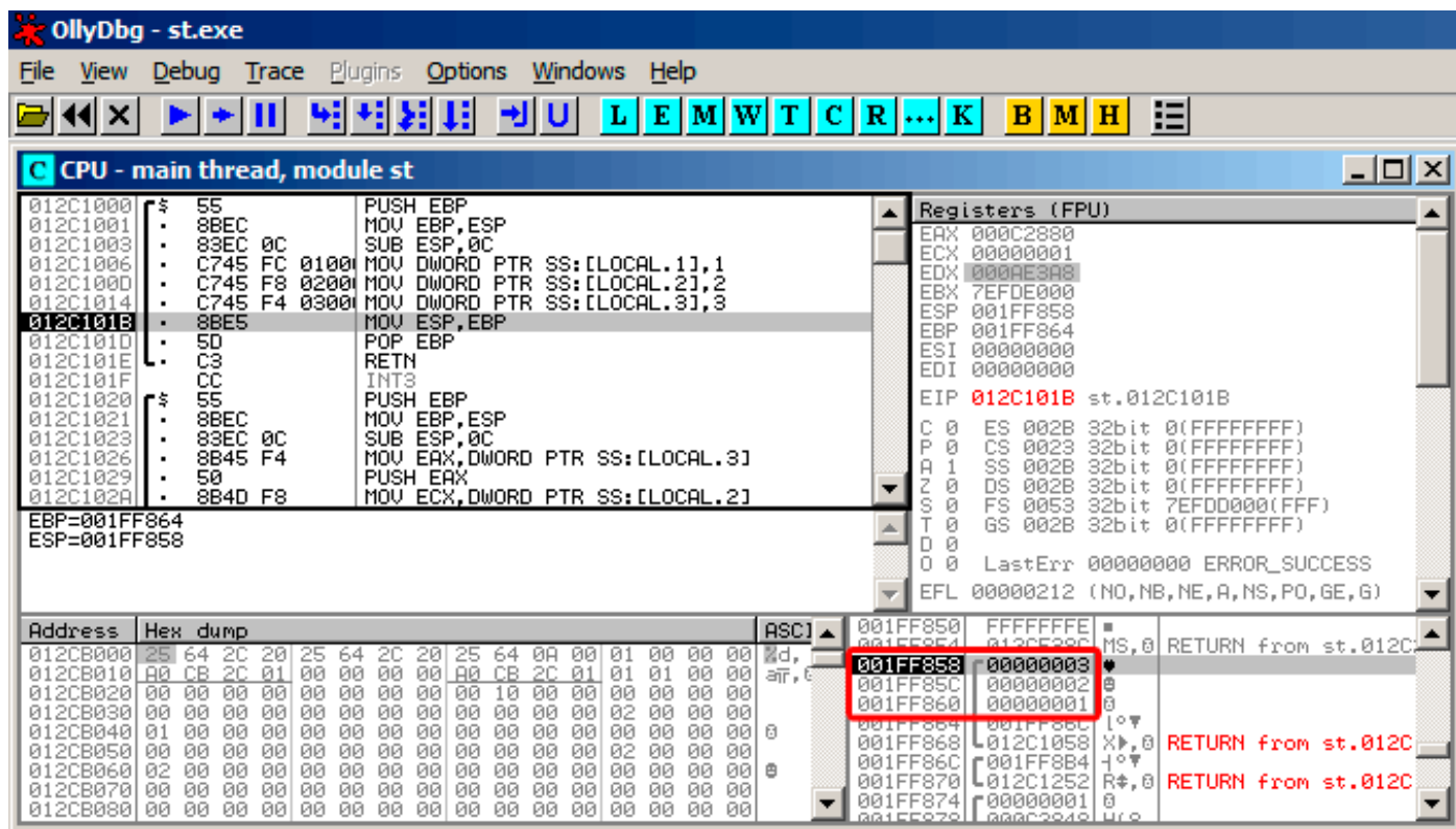
Figure 1.6: OllyDbg: f1()
