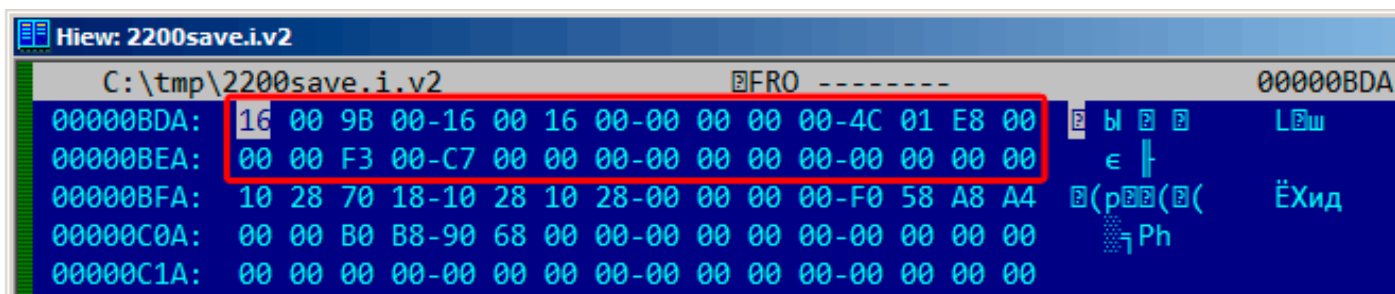
Figure 9.16: Hiew: state 1
