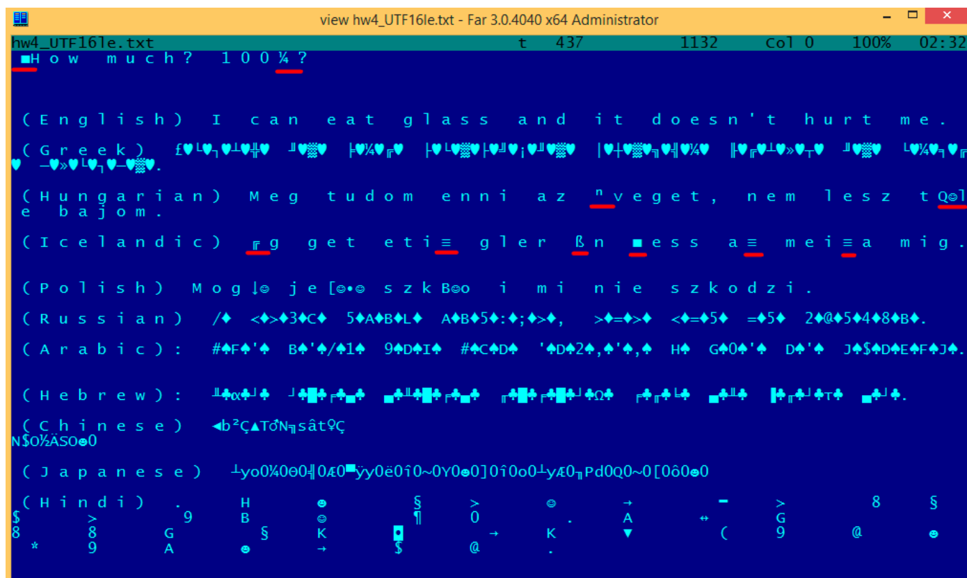
Figure 5.6: FAR: UTF-16LE
